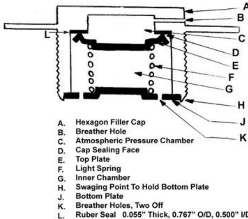
Early Post War Brake Master Cylinder Filler Cap and Breather Assembly
